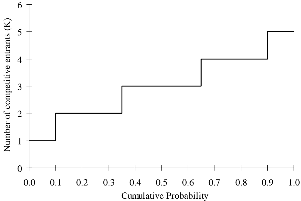
Figure 2.2. Inverse cumulative probability curve for number of entrants ( \mathbf{K} ).
