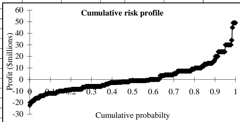
Figure 2.11. A simulation model with three random variables affecting profit.
