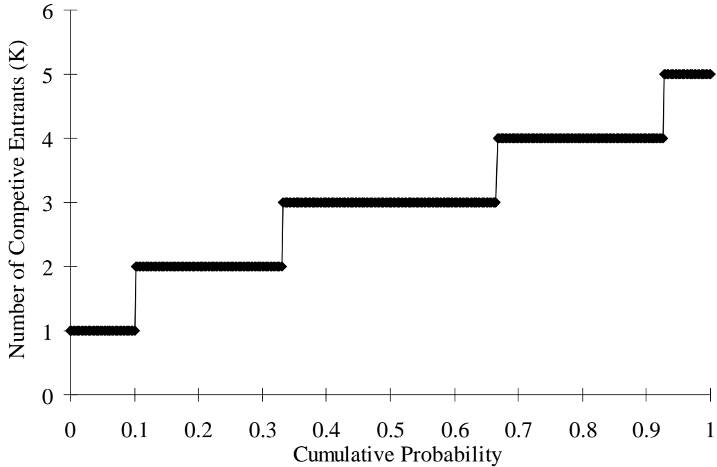
Figure 2.7. Estimate of an inverse cumulative distribution from simulation data.
