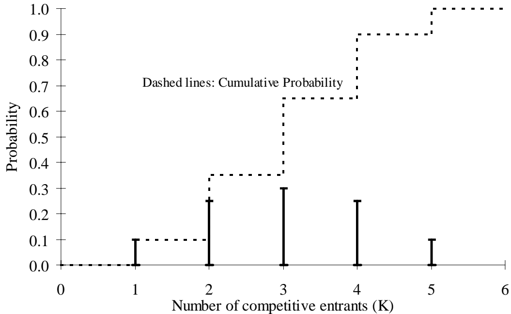
Figure 2.1. Discrete Probability Distribution for the Number of Entrants (K).
