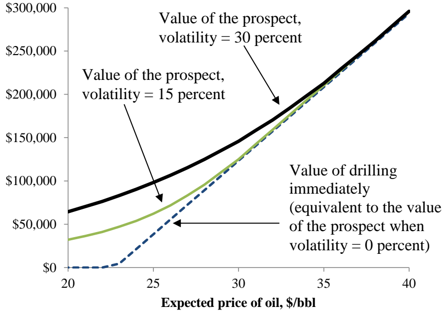
Figure 8: Comparison of the value of holding a drilling prospect to the profits from drilling
