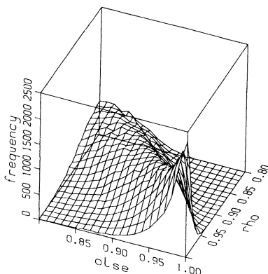
FIGURE 1.—Joint frequency distribution of \hat{\rho} and \rho .
