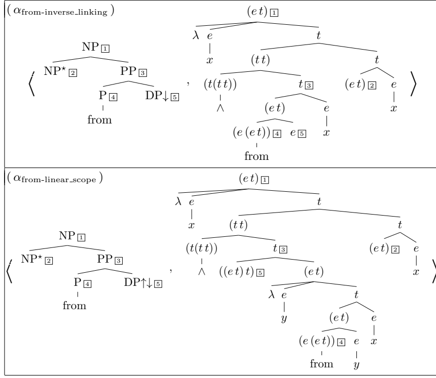
Fig. 5. The example coTAG G_{\text{scope}} (part 2)
