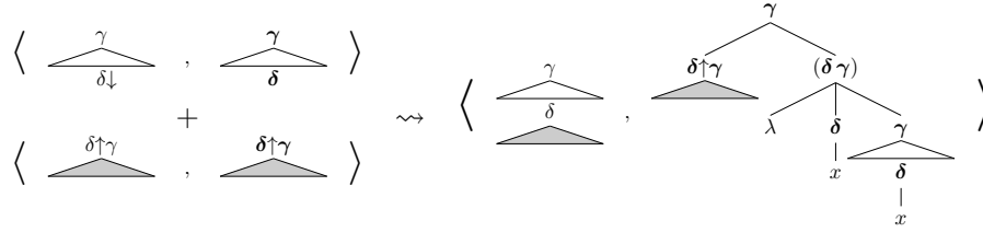
Fig. 3. Cosubstitution schematically: syntactically, tree with root-label \delta\uparrow\gamma is cosubstituted at leaf labeled \delta\downarrow in tree with root-label \gamma \in \mathit{Cat} ; while semantically, the corresponding tree with root-label \delta\uparrow\gamma is “quantified in” at the root of the corresponding tree with root-label \gamma .
