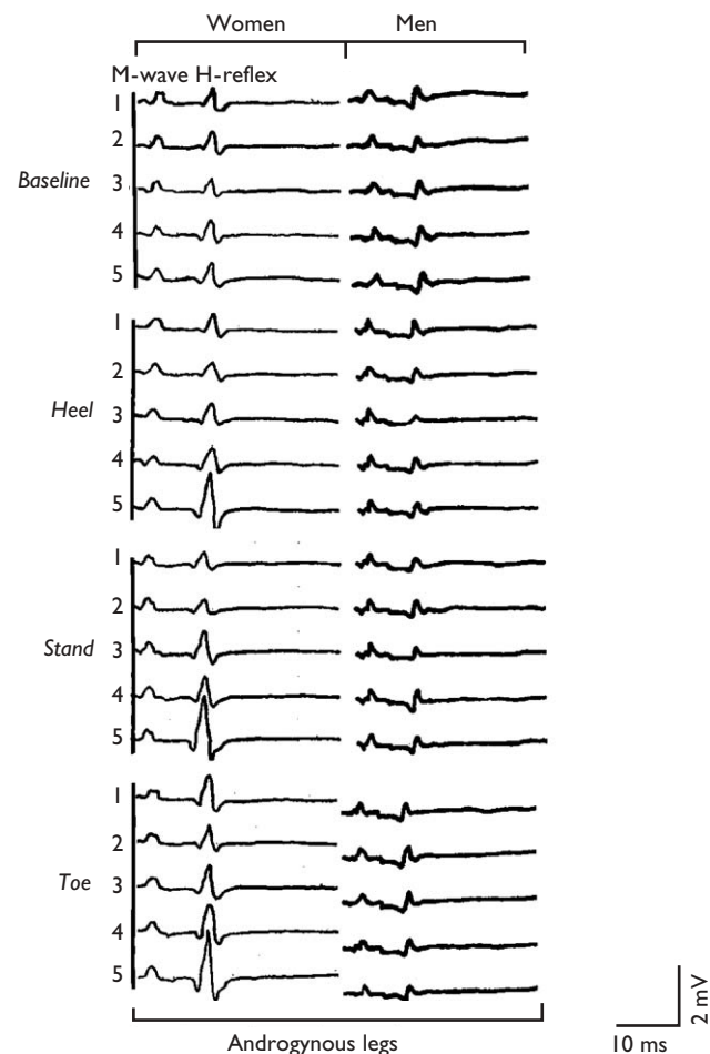
Fig. 1 The M-wave and H-reflex response in one female and one male participant during baseline and viewing heel, stand and toe.
