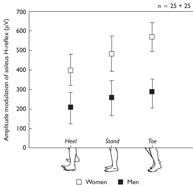
Fig. 2 Spinal excitability of left soleus H-reflex when watching bipedal step in the model of androgynous-appearing legs. No matter observing which kind of bipedal step, female participants (□) have significantly stronger amplitude modulation of H-reflex ( P = 0.024 ) than males (■). Additionally, their spinal excitability mimics the observed bipedal step, that is, the amplitude modulation of soleus H-reflex during their observation increases from heel, stand, to toe. Heel, bipedal heel-stepping; stand, standing still; toe, bipedal toe-stepping. Error bars indicate SEM.
