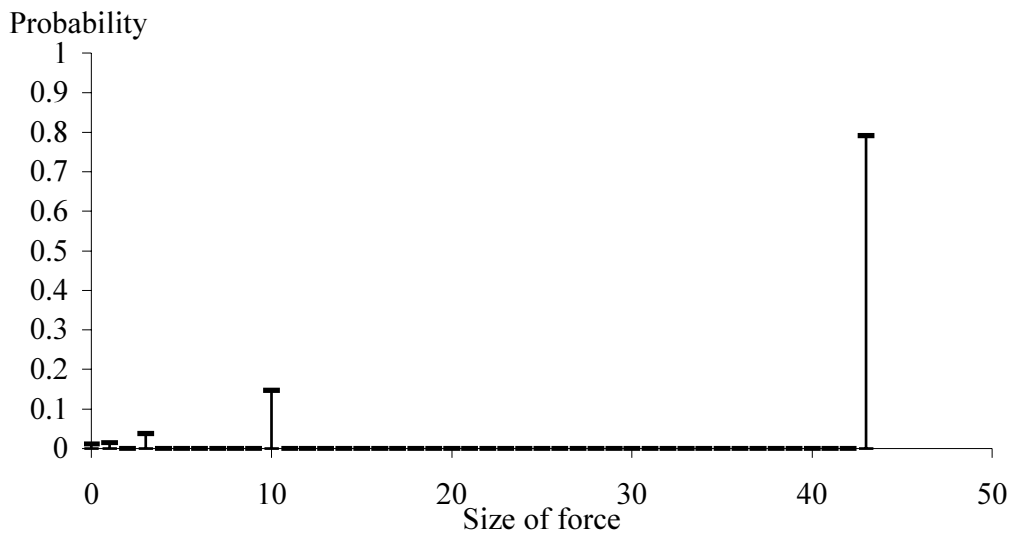
Figure 4. Discrete (integer) approximation of the randomized negotiation-proof equilibrium, for an example with R=90 , \delta=0.05 , \lambda=0.2 , c=5 , and s=3 .
